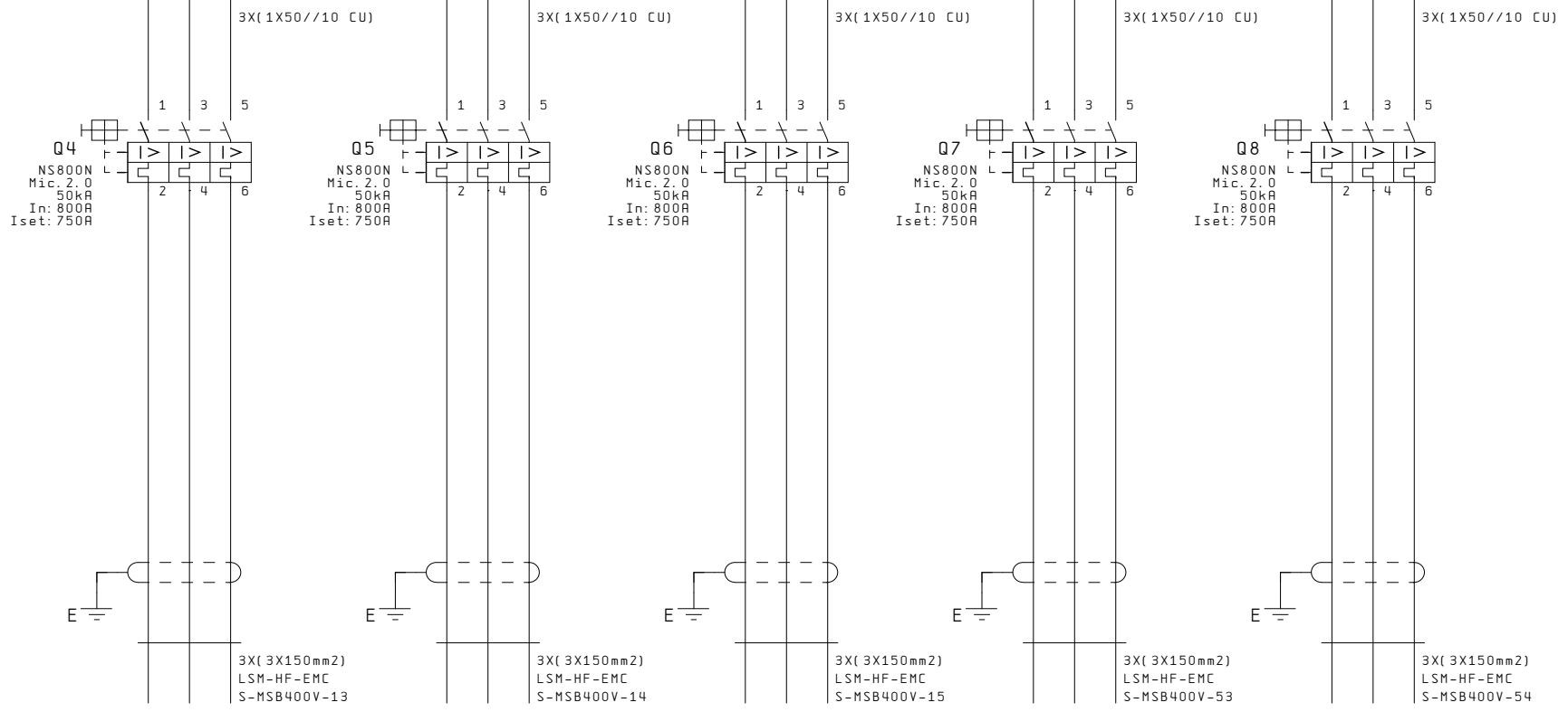
NO.5 400VAC DAGITIM PANELI
